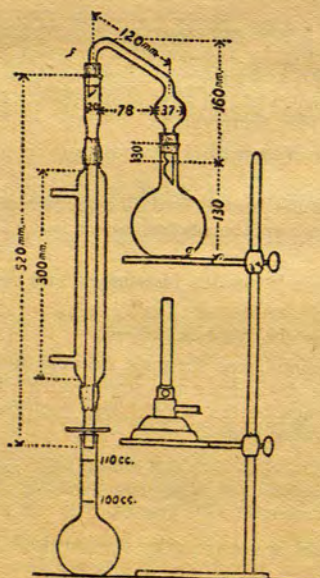
APPARATUS FOR DETERMINATION OF POLENSKE VALUE
