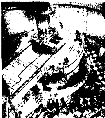
Interior view of Canada-India Atomic Reactor, 'Cirus' at Trombay near Bombay.
