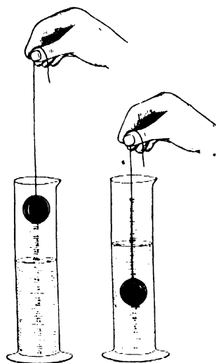
Fig. 3-11 Measuring the volume of a solid
