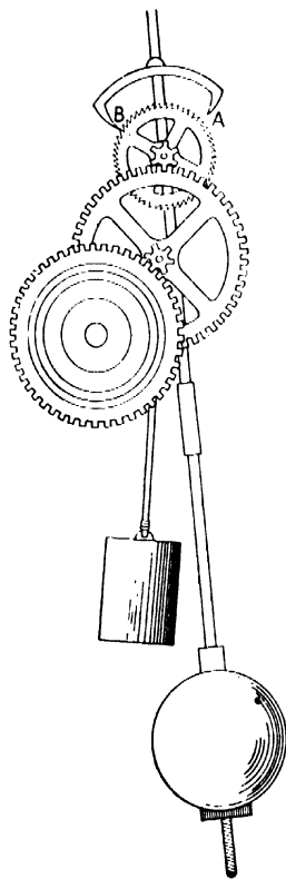
Fig. 4—11, The escapement mechanism in a pendulum clock
