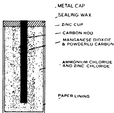
Fig. 8—2 A dry-cell (battery).
