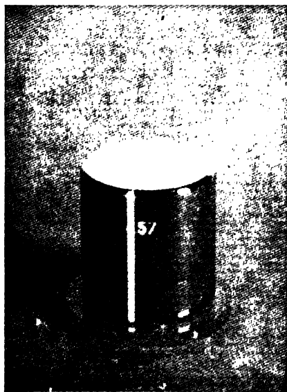
Fig. 7—7 (b) Prototype kilogram kept at National Physical Laboratory, New Delhi.
