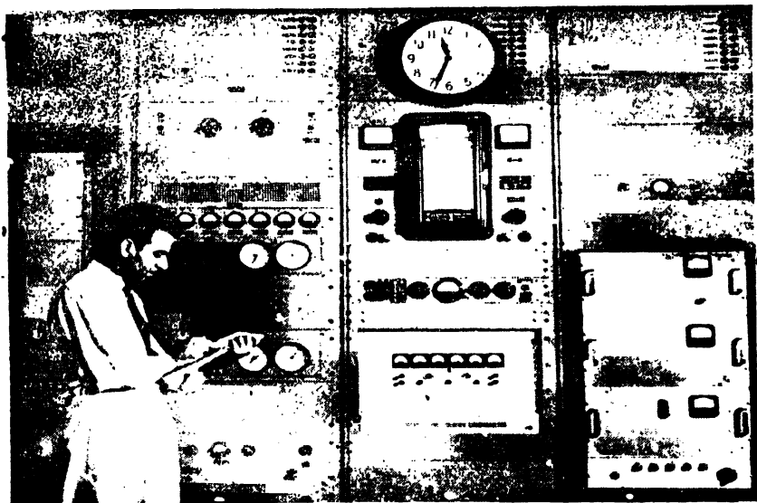
Time and Frequency standards at National Physical Laboratory, New- Delhi, which measures time to an accuracy of 1 part to 10^8 sec.
