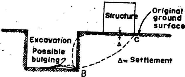
Settlement caused by excavation (BC is the sliding surface)
