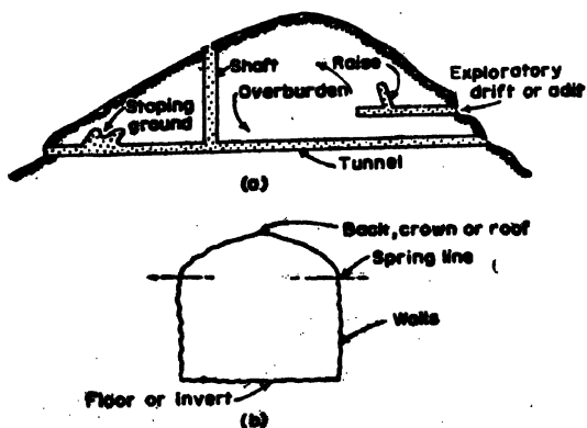
Tunnel terminology
