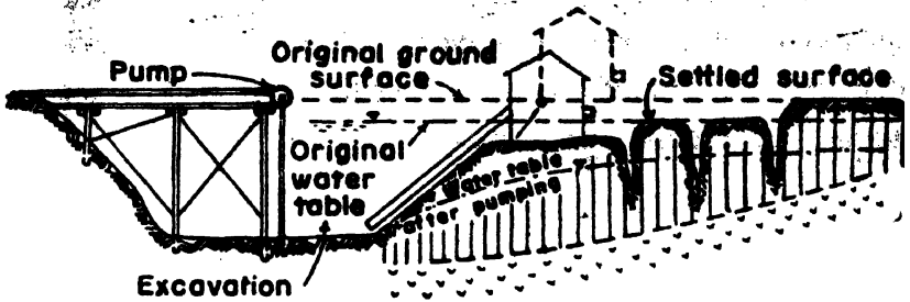
Settlement and cracking due to pumping.
