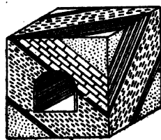
(f) OBLIQUE STRATA (PRESSURE CONCENTRATION ON SIDES)
