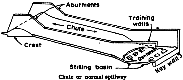
Chute or normal spillway
