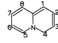
4H-Quinolizine
