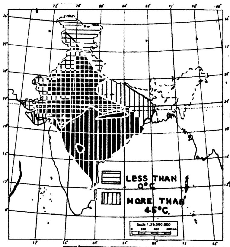
Map 3 Areas of Highest and Lowest Temperatures recorded
