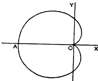
(ii) r = a(1 - \cos \theta) .
