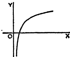
(i) y = \log x .
