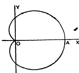
(i) r = a(1 + \cos \theta) .
